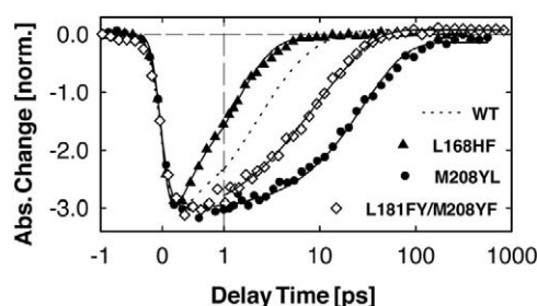
FIGURE 2 Transient absorption data (circles, triangles, diamonds) of different mutants and WT RC at 1050 nm (mutant L168HF, where the Q_Y absorption peak is blueshifted at the corresponding wavelength 1020 nm). The solid curves are modeled using a biexponential decay. The modeled time constants \tau_{1A} and \tau_{1B} (see Eq. 1) and their amplitudes are given in Table 2. Note the linear scale for the delay times of <1 ps and the logarithmic scale at later delay times.
